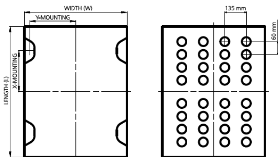
Ejector and mounting EUROMAP 2
