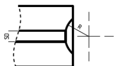
Ejector and mounting EUROMAP 2
